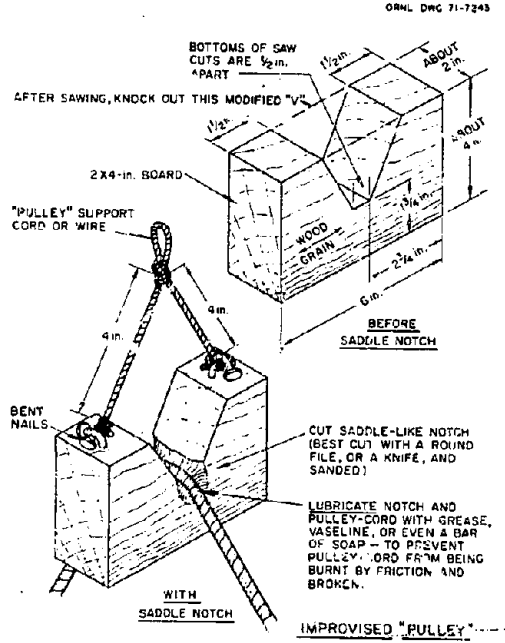
Fig. B-18. Improved pulley with saddle notch.
